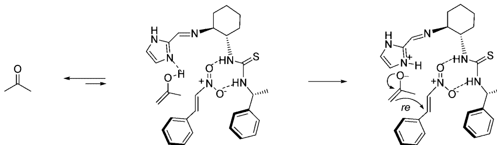
Scheme 4. Proposed transition state.
